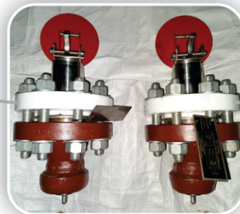
Pig Signallers (Intrusive Type)
